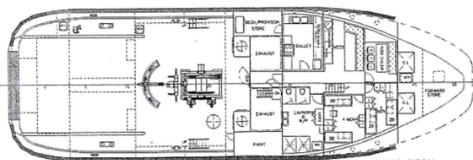
MAIN DECK
