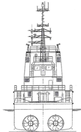
STERN VIEW
