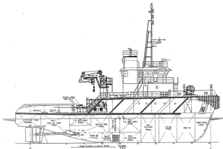
OUTBOARD PROFILE
