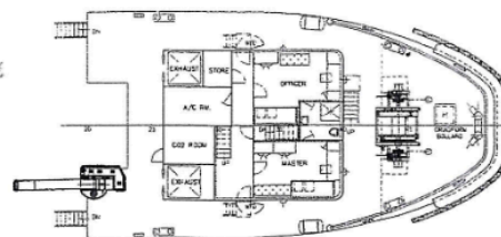
FORECASTLE DECK
